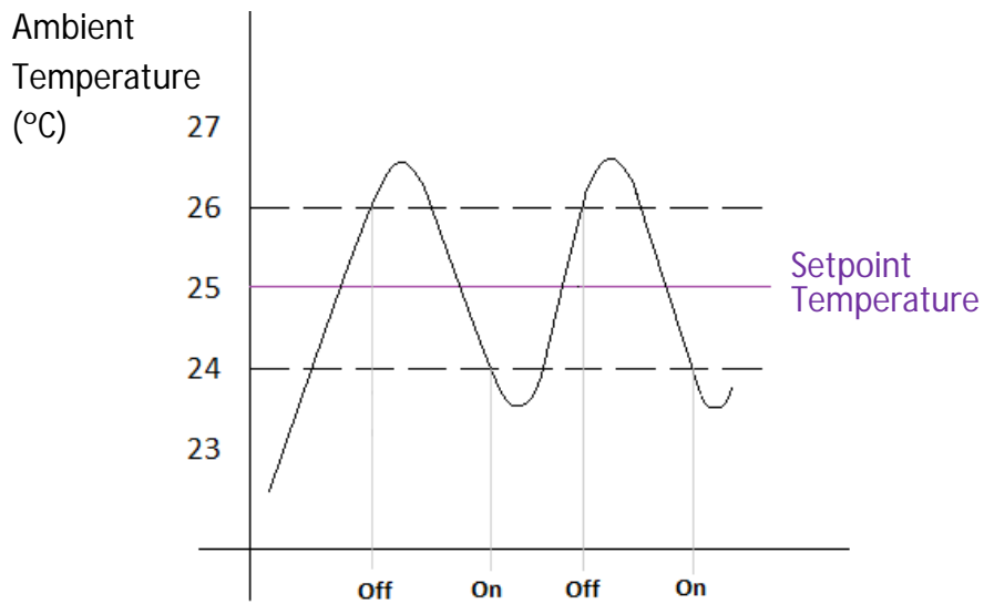
Figure 2.1. Typical graph of 2 point with hysteresis system
