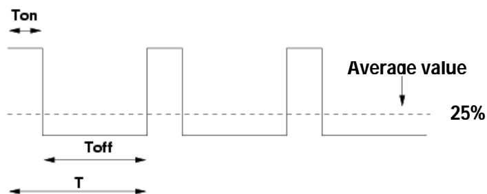
Figure 2.4. Value of variable PI equal to 25%
