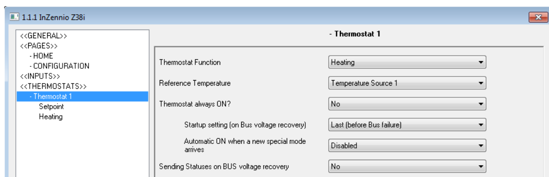
Figure 3.2. General configuration window of the thermostat, by default
