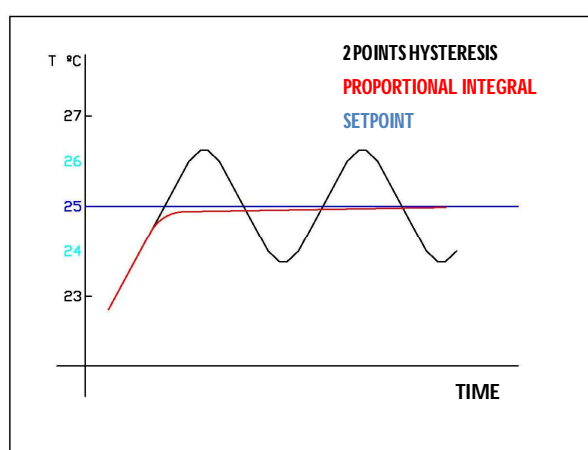
Figure 2.6. Ideal comparison: PI control vs. 2 point control
