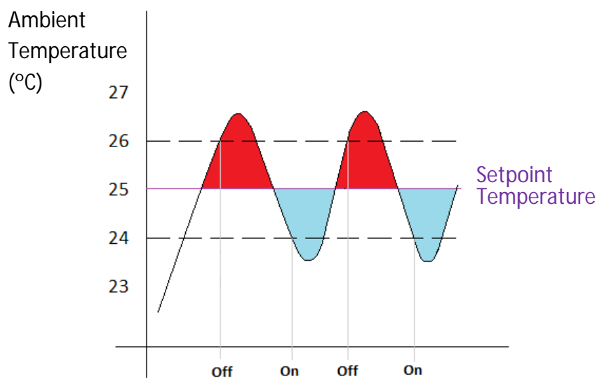
Figure 2.2. Inefficiency of 2 point control
