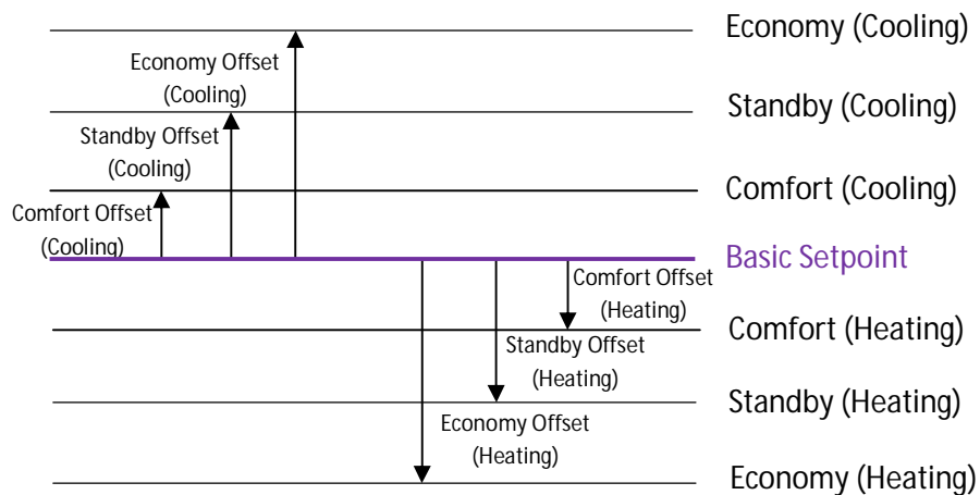
Figure 2.10. Relative setpoints. Cooling and Heating mode
