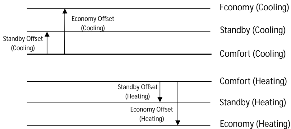
Figure 2.9. Absolute setpoints. Cooling and heating mode
