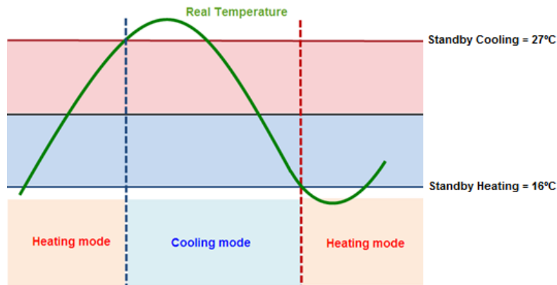
Figure 4.1. H/C Automatic Switching example
