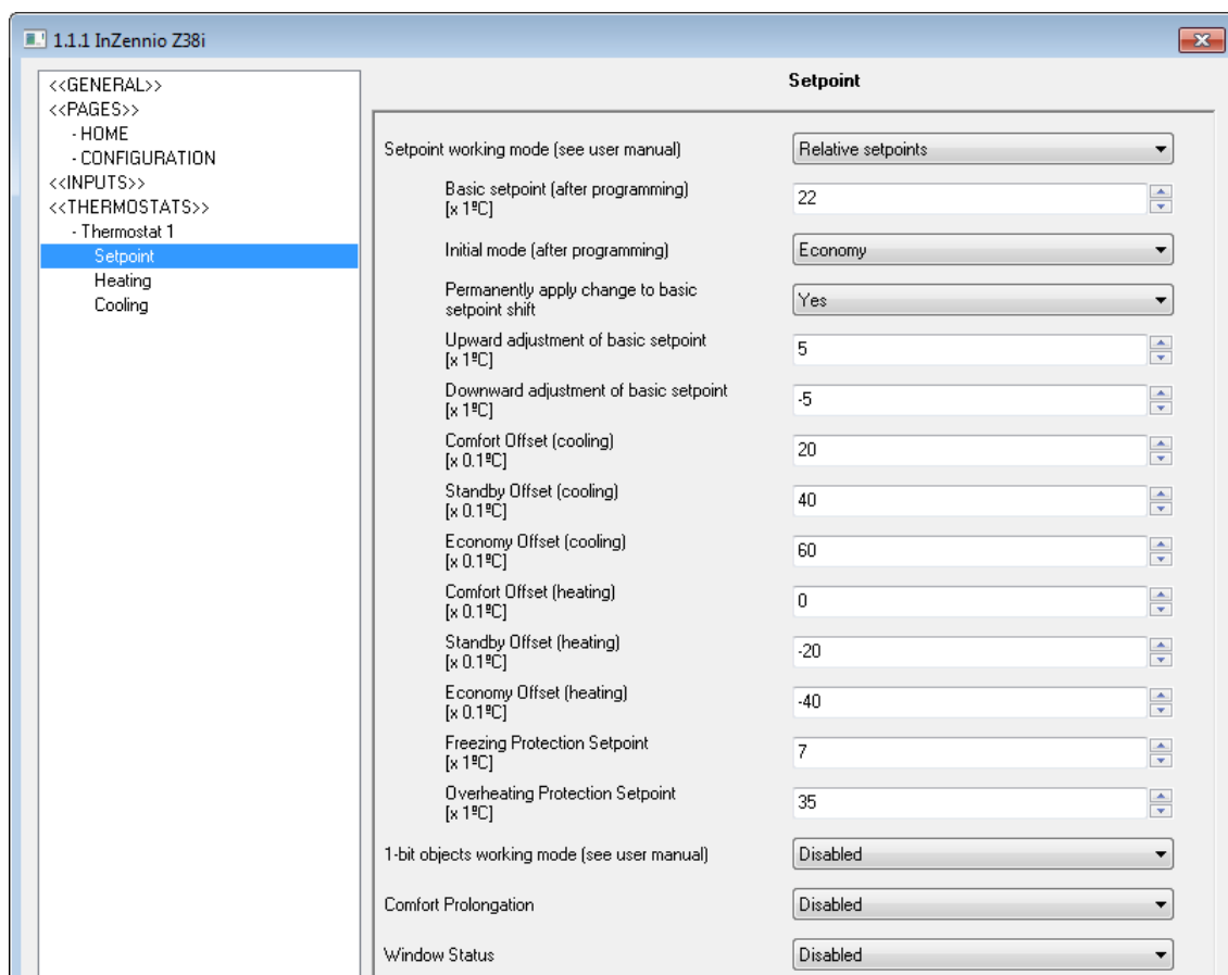
Figure 3.4. Parameters of the Relative setpoints method
