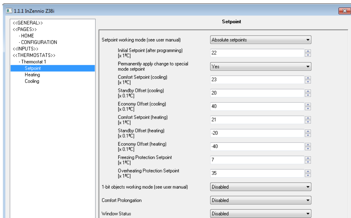
Figure 3.3. Parameters of the Absolute setpoints method
