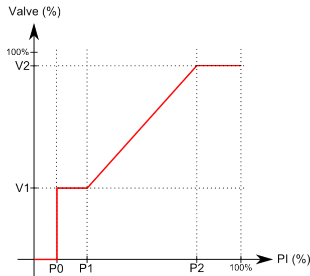
Figure 4. Control order scaling diagram
