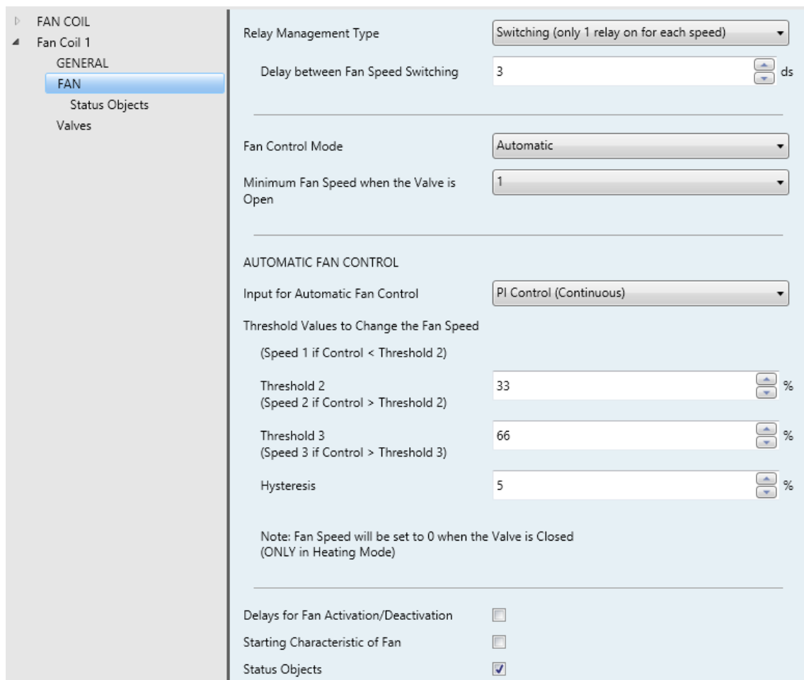
Figure 5. Valve-oriented control: Fan
