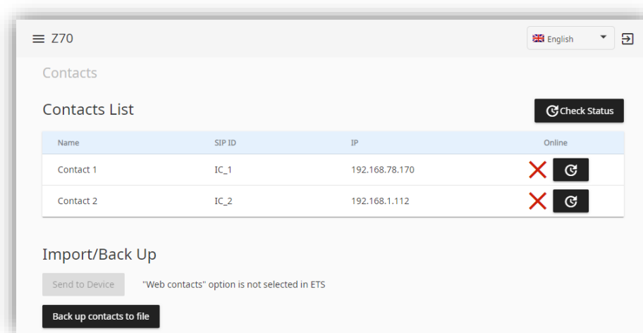
Figure 6. Contacts tab (From ETS)
