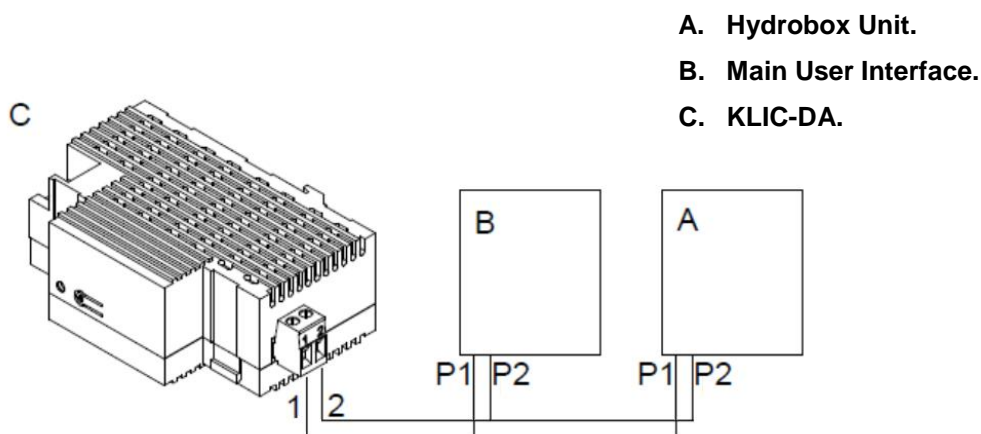
Figure 3. Connection to the P1/P2 bus
