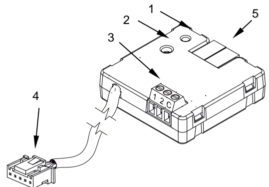
Figure 1: KLIC-MITT v2
