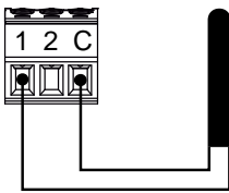
Zennio temperature probe.
