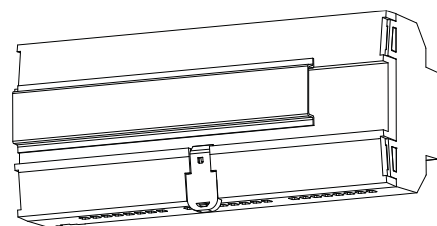
Figure 3: Mounting MAXinBOX 24 on DIN rail
