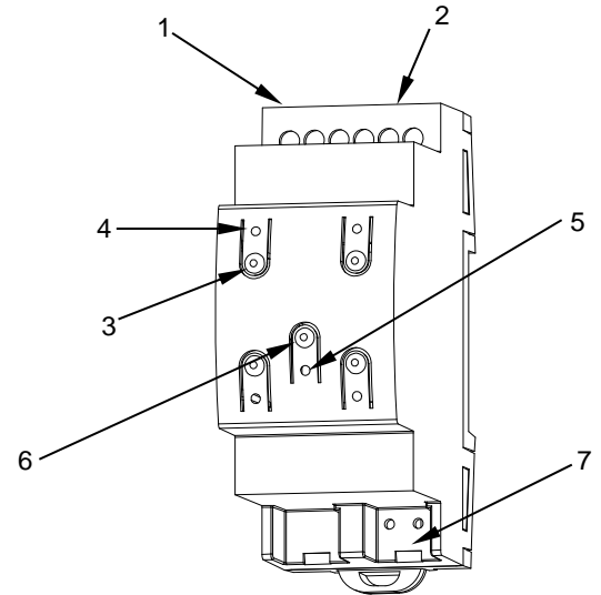
Figura 1: HeatingBOX 230V 4X
