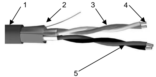
Figure 1. 2 x 2 x 0.8mm KNX cable
