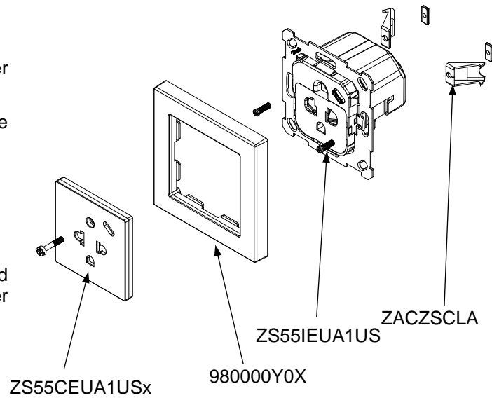
Figure 1. Euro-American socket insert with USB type C
