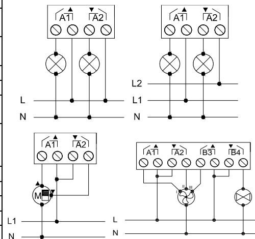
Figure 2: Wiring example (from left to right, and up to down): 2 loads, 2 loads connected to different phases, shutter and fan coil
