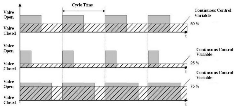
Figure 9. PI-PWM Control
