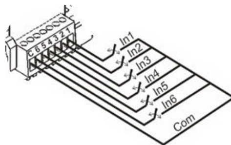
Figure 5. Inputs
