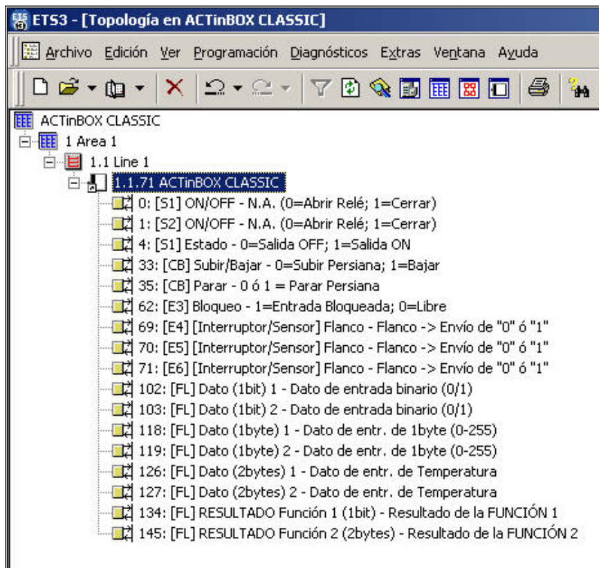
Figure 1. Communication Objects
